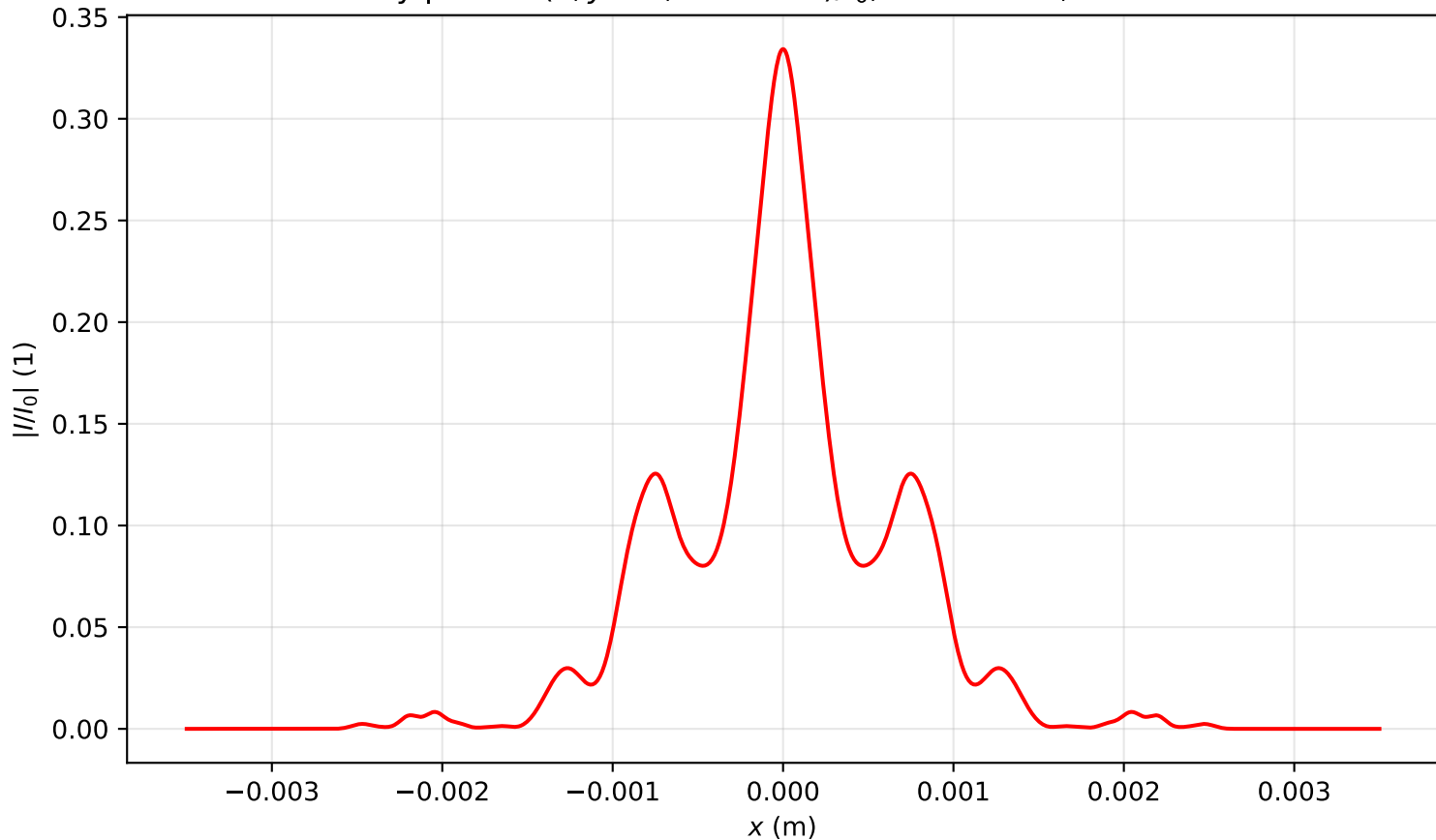
Intensity profile I(x, y = 0, z = 2.149)/I_0 , P_{in}=6.0P_{cr} , artificial time
